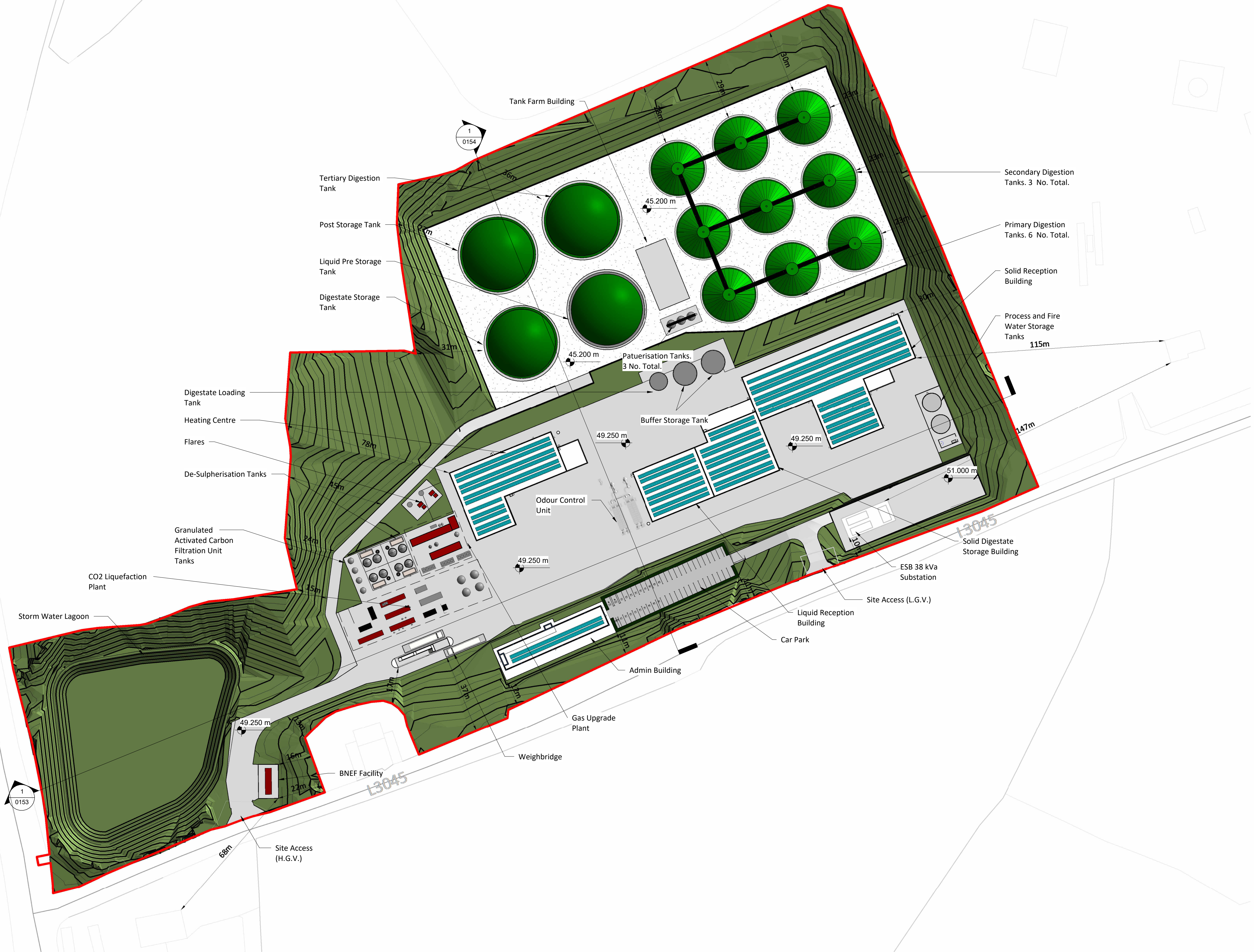
PROPOSED SITE LAYOUT PLAN Scale 1 : 1000
